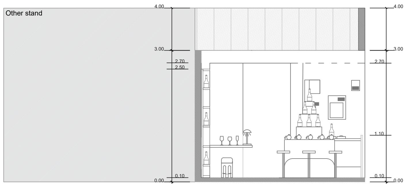
SECTION BB'
